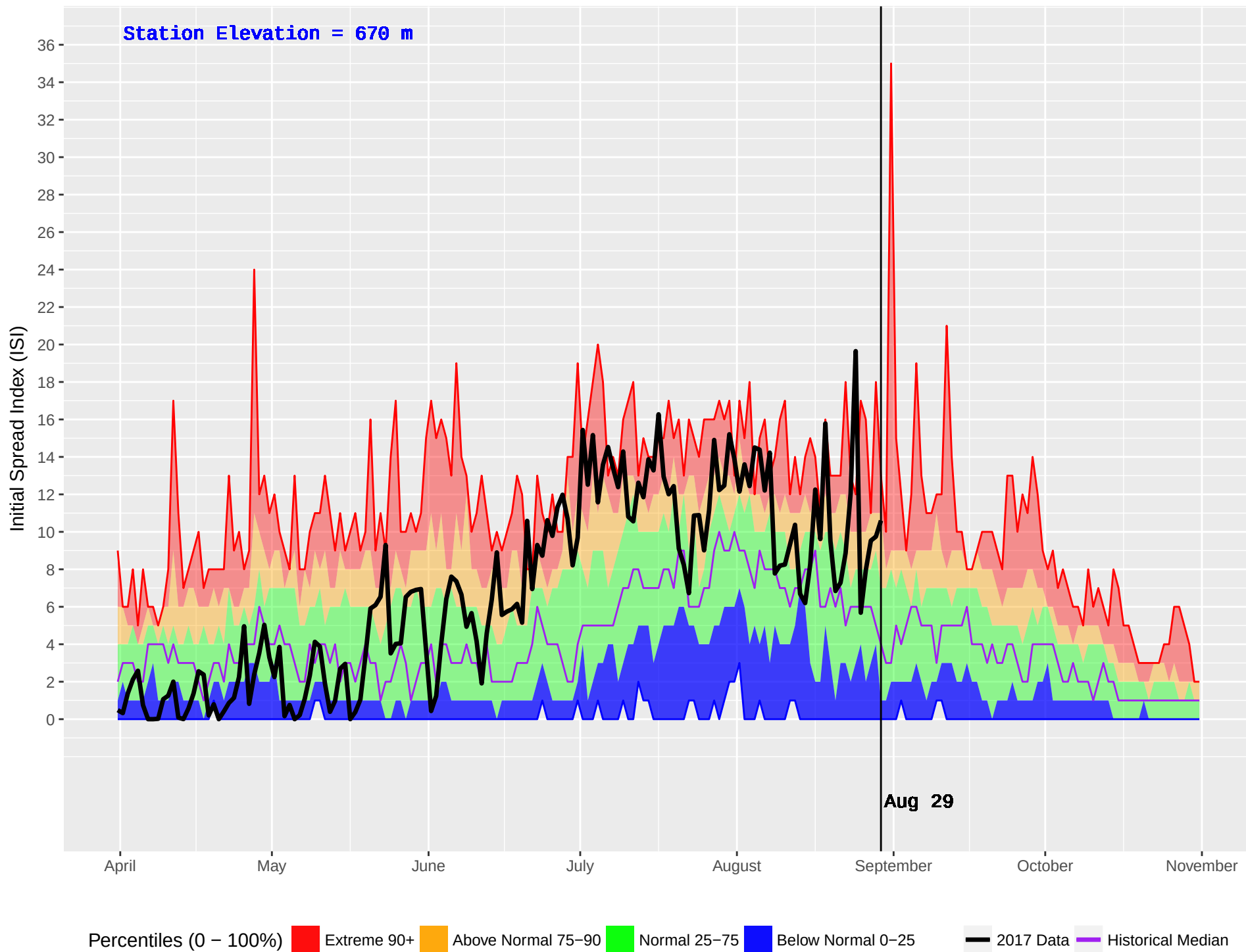
FINTRY (298) : Historical (1989–2016) and Current (2017) Noon Initial Spread Index (ISI)
