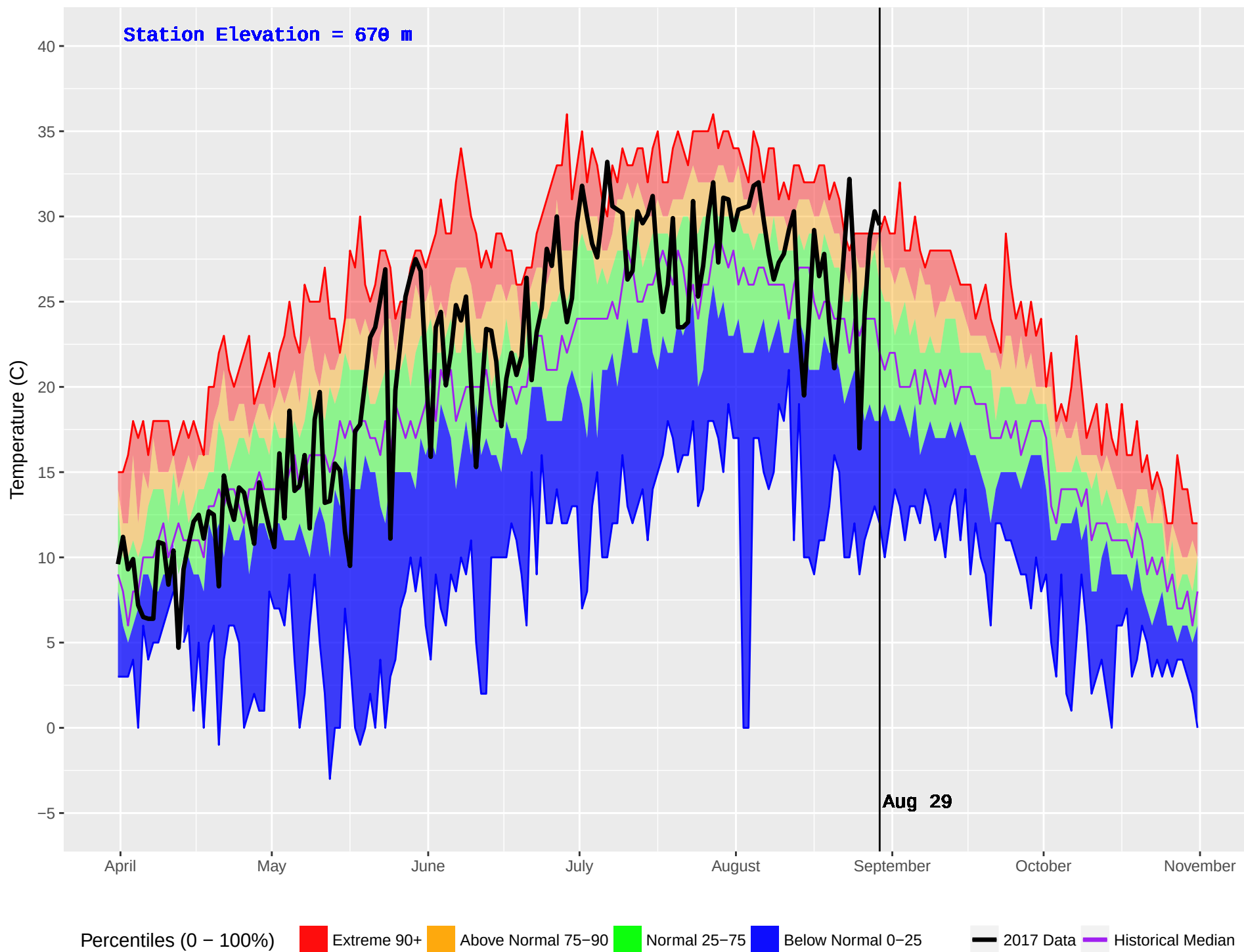
FINTRY (298) : Historical (1989–2016) and Current (2017) Noon Temperature
