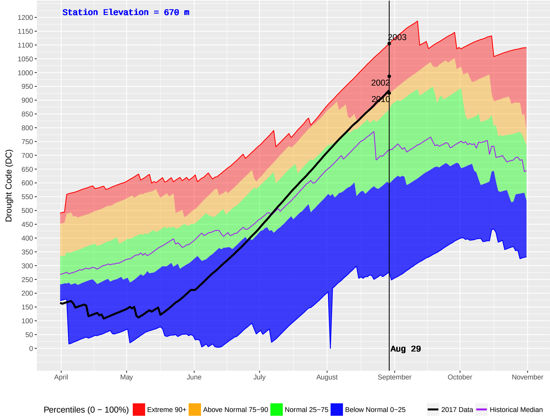
FINTRY (298) : Historical (1989–2016) and Current (2017) Noon Drought Code (DC)
