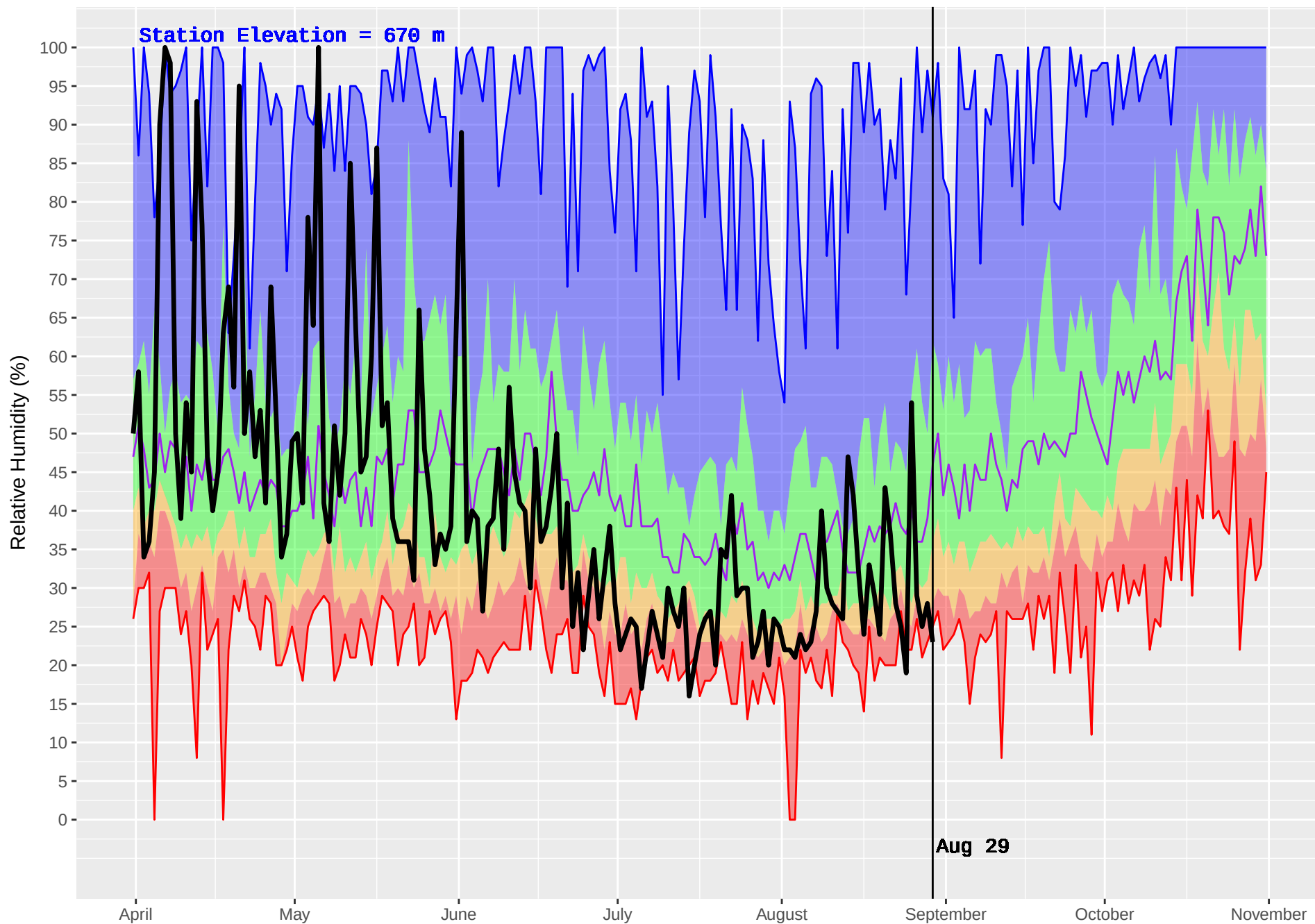
FINTRY (298) : Historical (1989–2016) and Current (2017) Noon Relative Humidity
