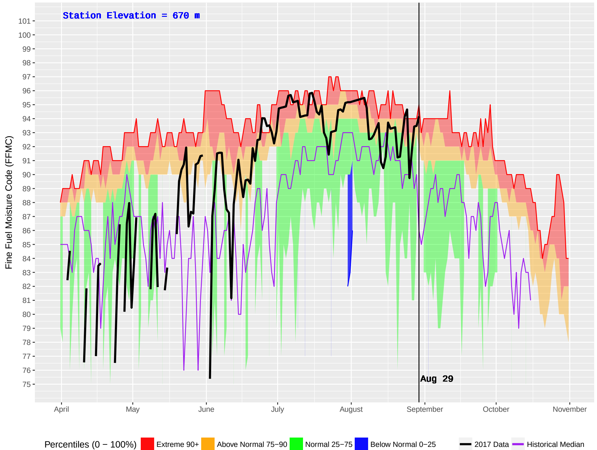
FINTRY (298) : Historical (1989–2016) and Current (2017) Noon Fine Fuel Moisture Code (FFMC)
