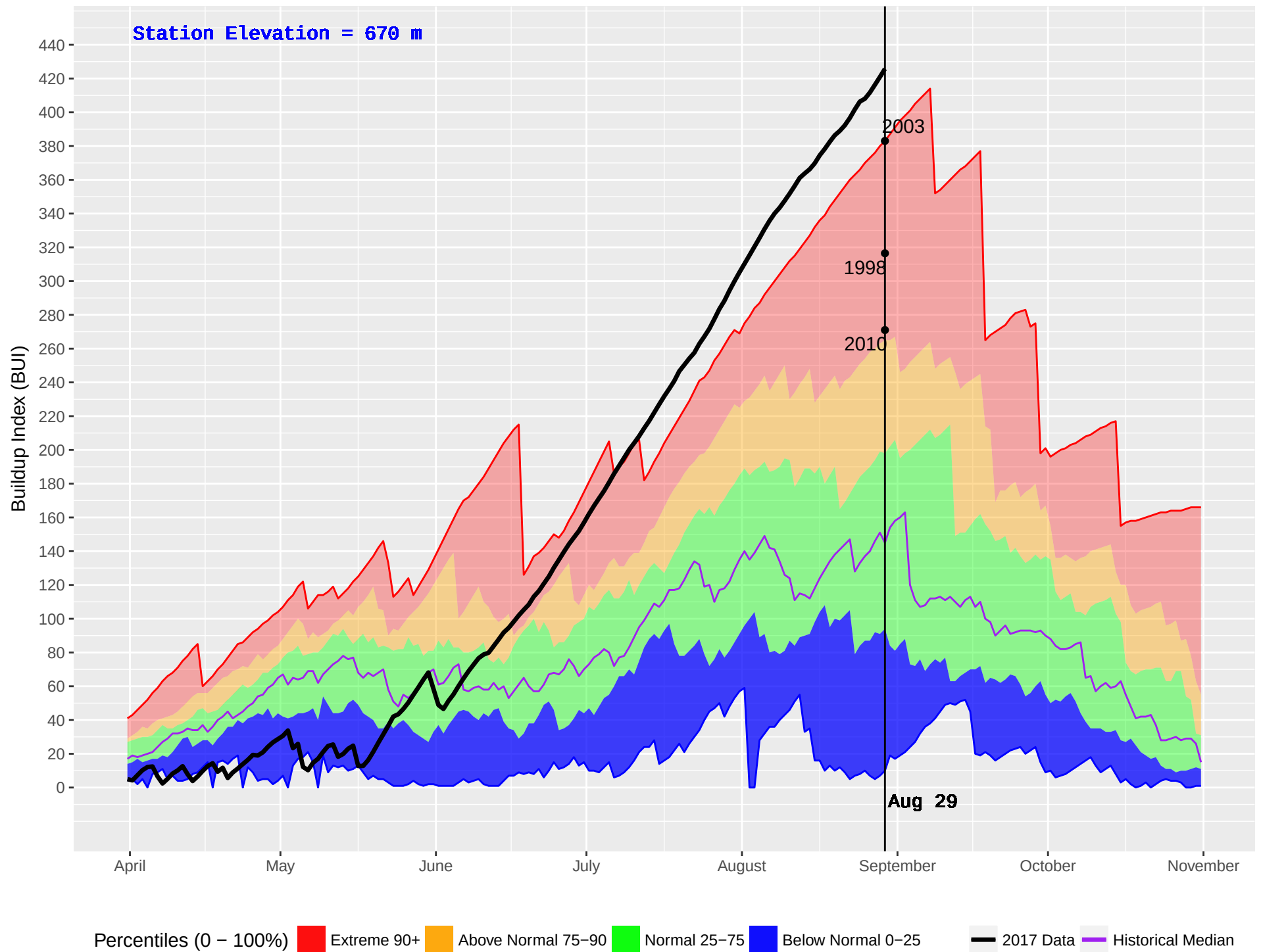
FINTRY (298) : Historical (1989–2016) and Current (2017) Noon Buildup Index (BUI)
