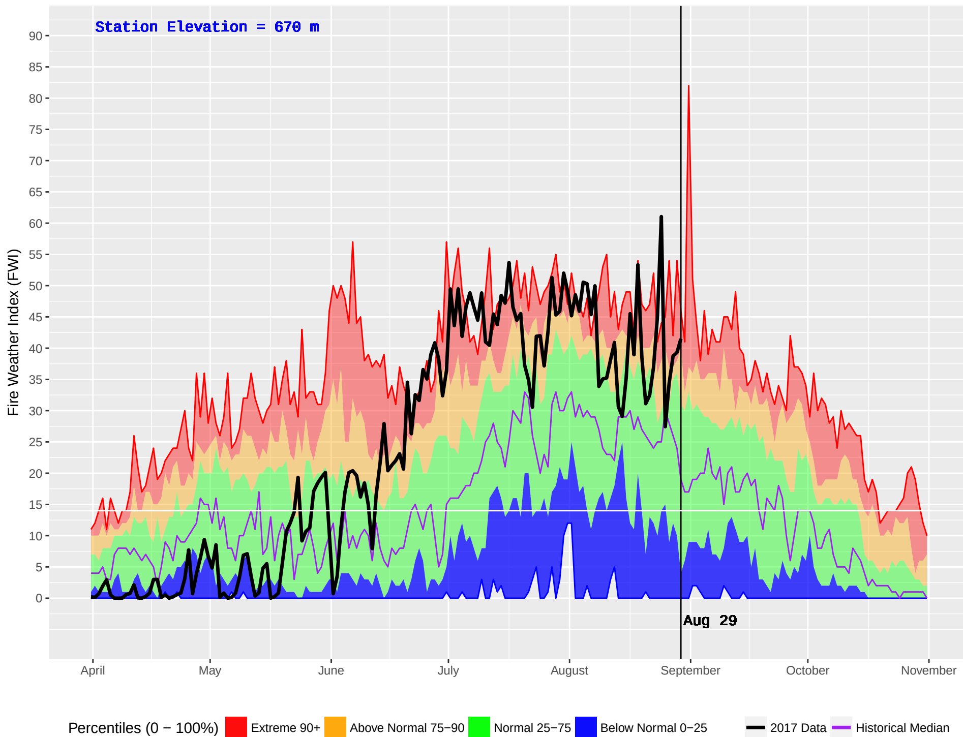
FINTRY (298) : Historical (1989–2016) and Current (2017) Noon Fire Weather Index (FWI)
